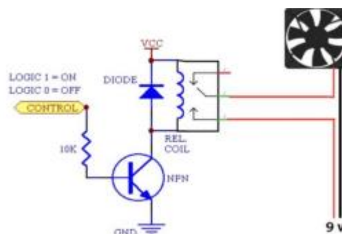
Fig. 3: Relay Connections.
